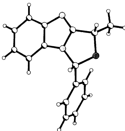
Figure 2. X-Ray crystal structure of 18.
