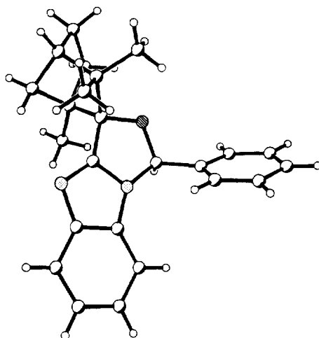
Figure 1. X-Ray crystal structure of one of the independent molecules of 13 .
